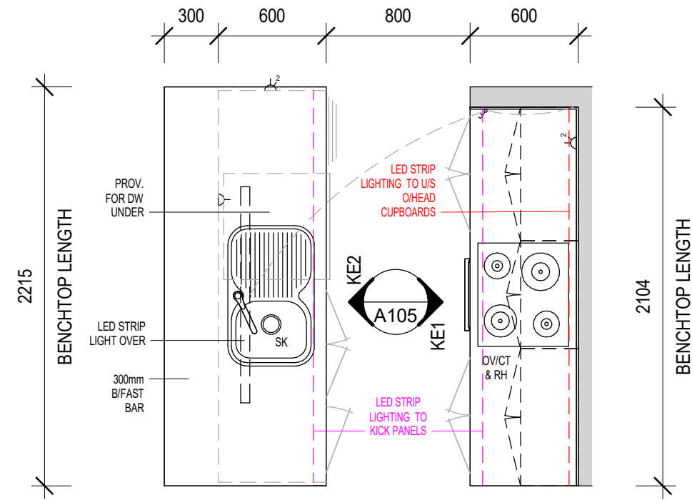
KITCHEN PART A - PLAN VIEW
