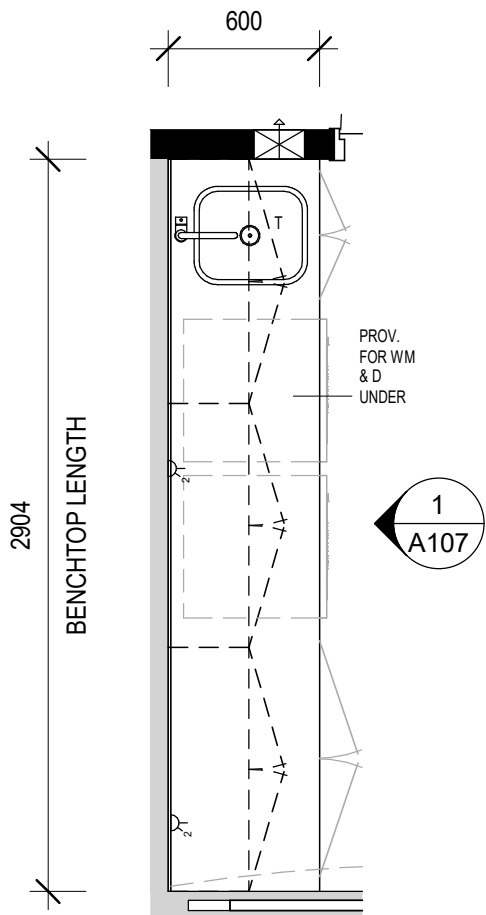
LAUNDRY - PLAN VIEW
