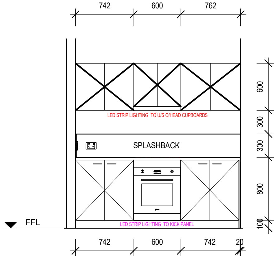
KITCHEN ELEVATION 1 (KE1)
