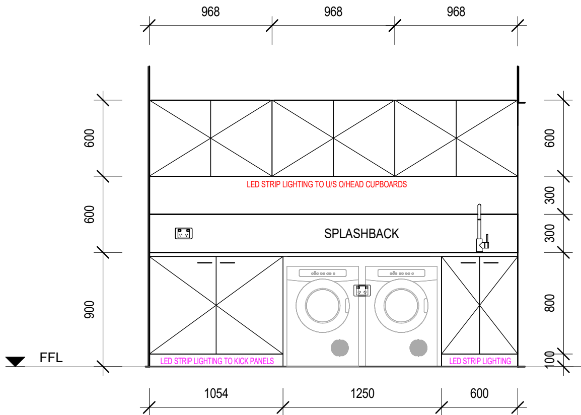
LAUNDRY ELEVATION (LE)
