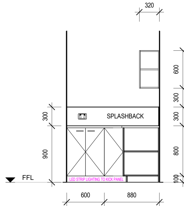
KITCHEN ELEVATION 3 (KE3)
