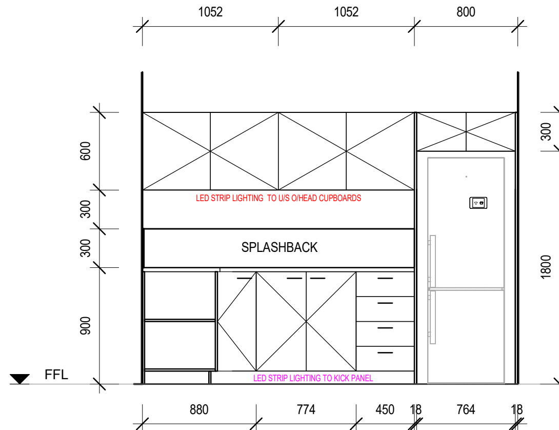
KITCHEN ELEVATION 4 (KE4)
