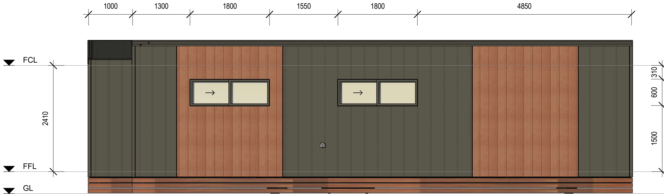
FRONT ELEVATION (1)
