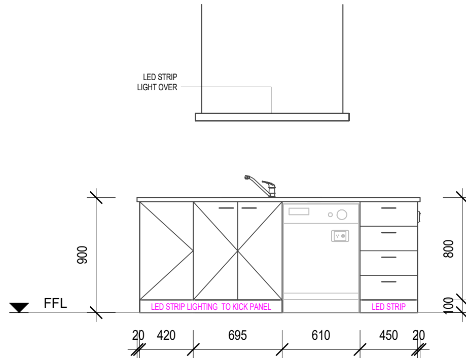
KITCHEN ELEVATION 2 (KE2)
