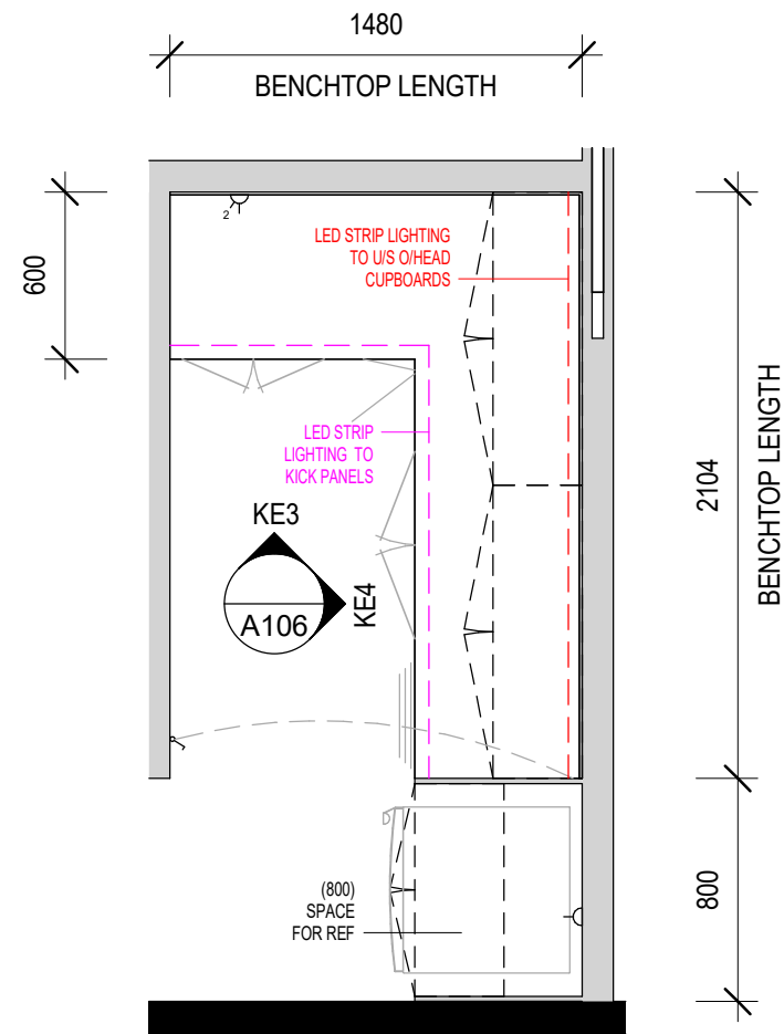
KITCHEN PART B - PLAN VIEW
