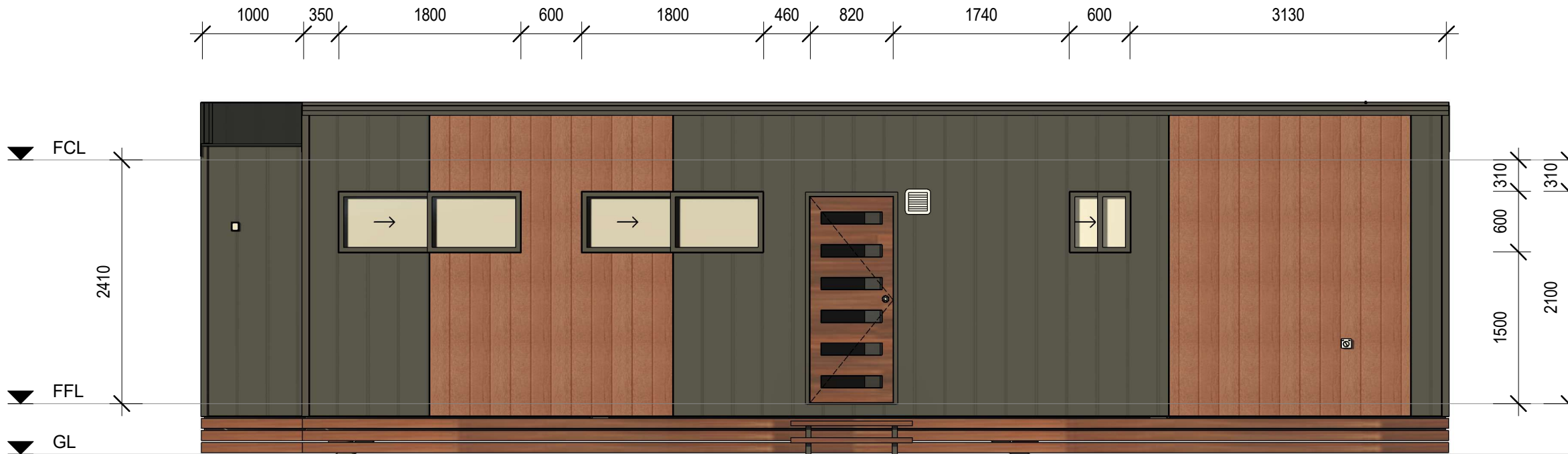
REAR ELEVATION (2)
