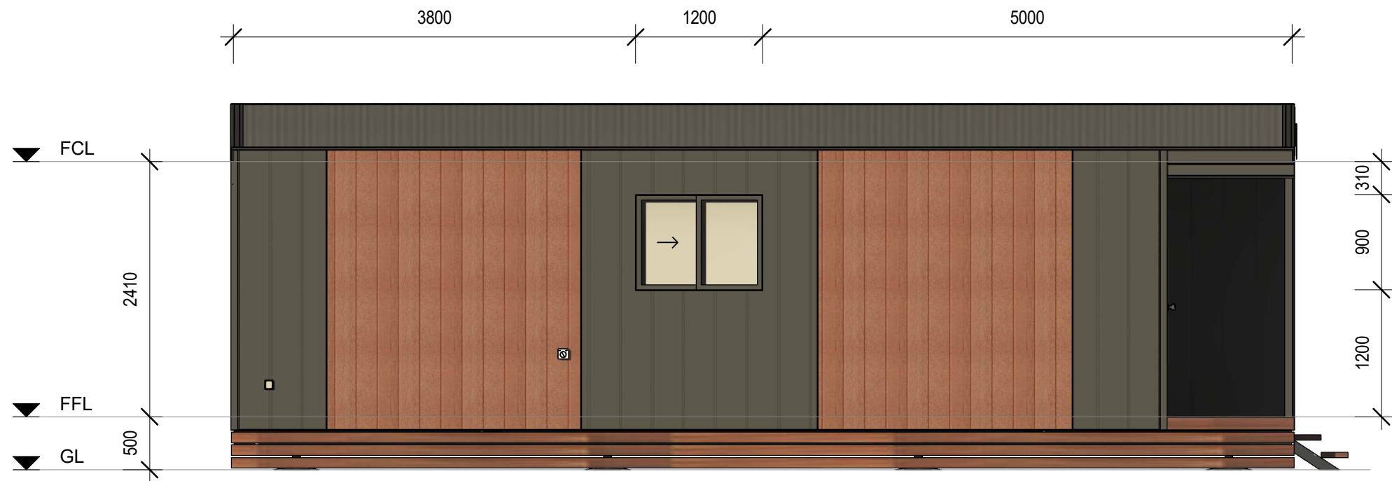
REAR ELEVATION (2)
