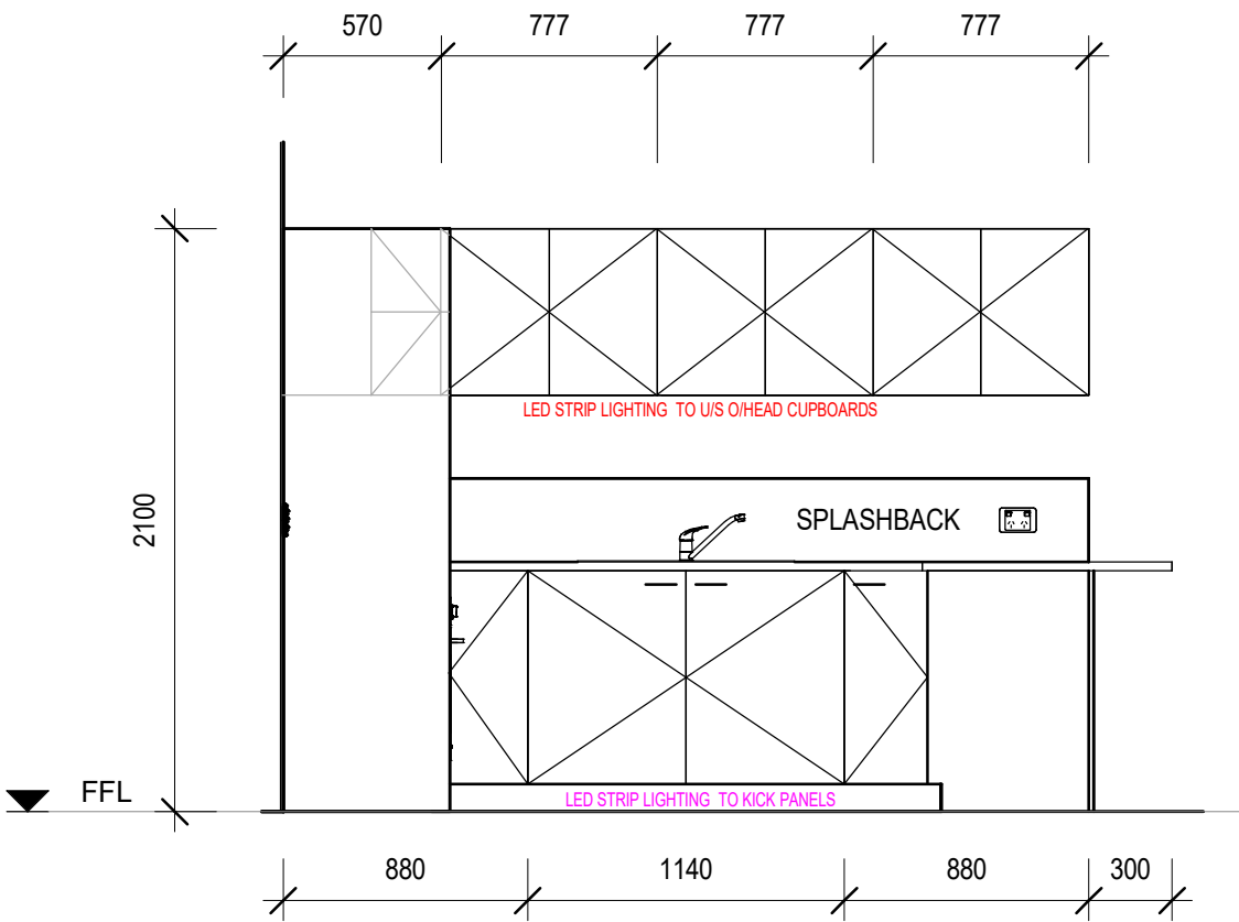
KITCHEN ELEVATION 1 (KE1)
