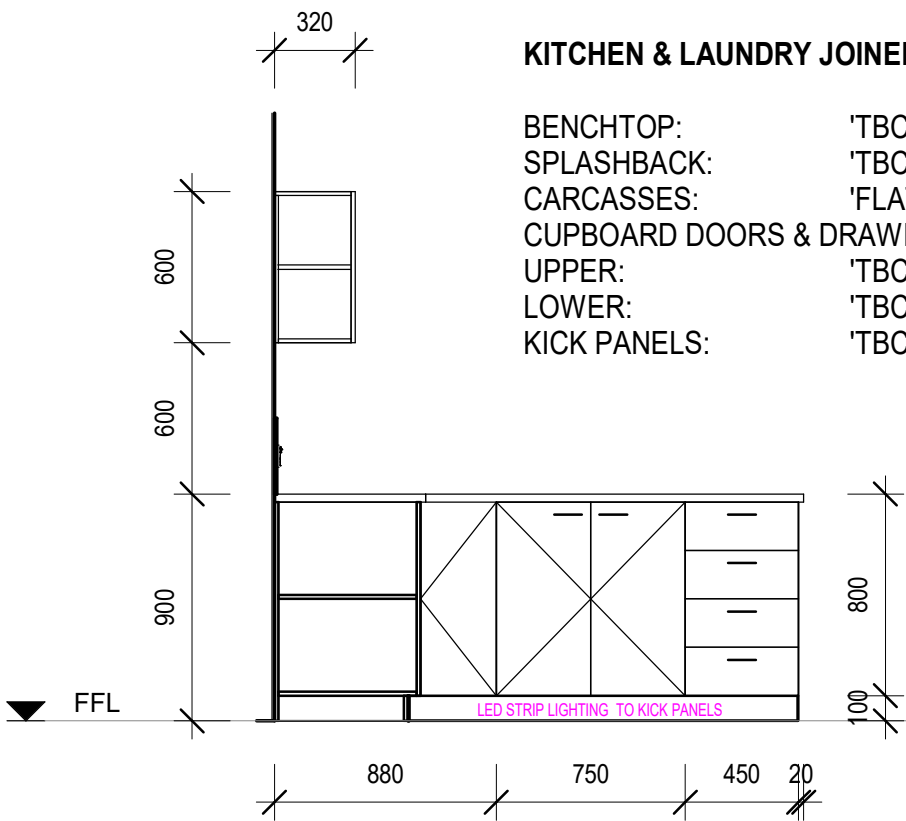
KITCHEN ELEVATION 3 (KE3)
