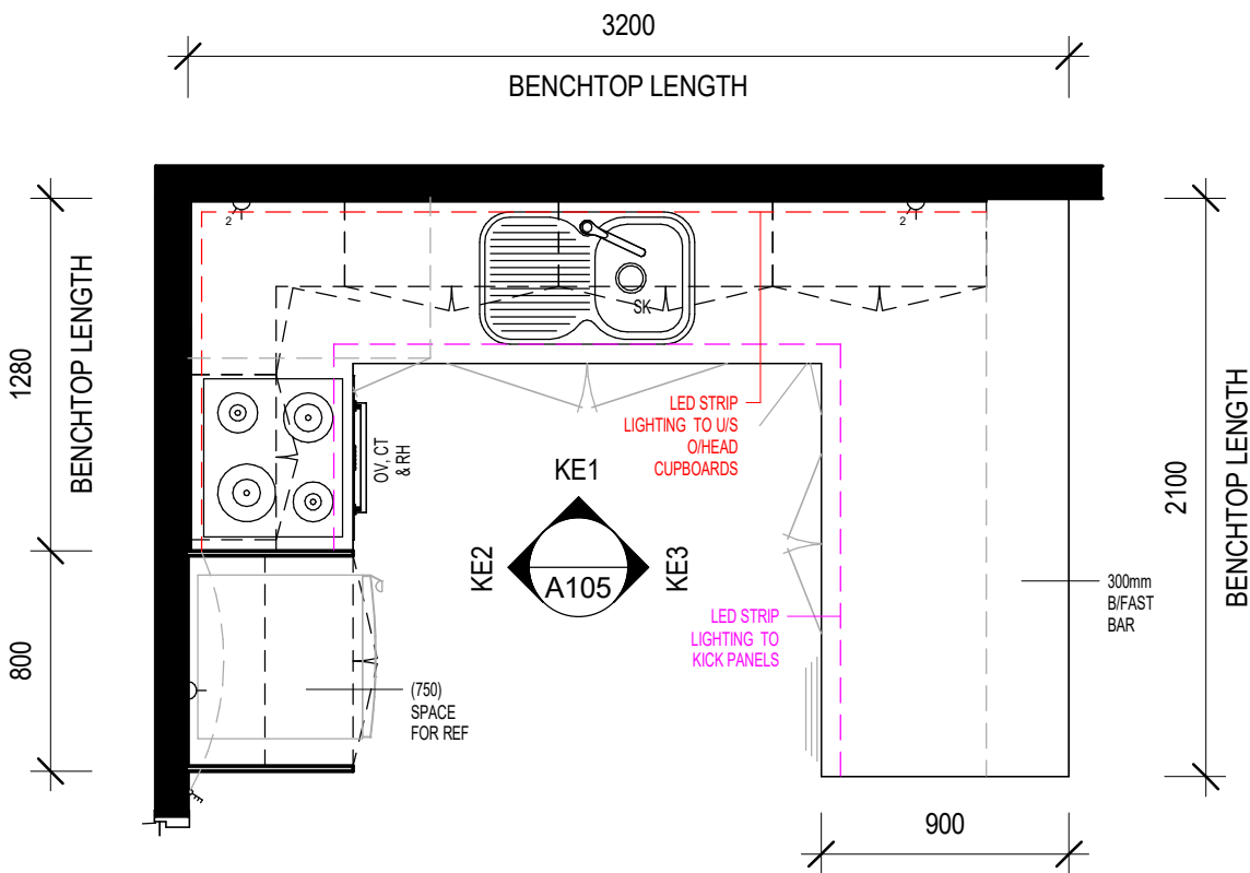
KITCHEN JOINERY - PLAN VIEW
