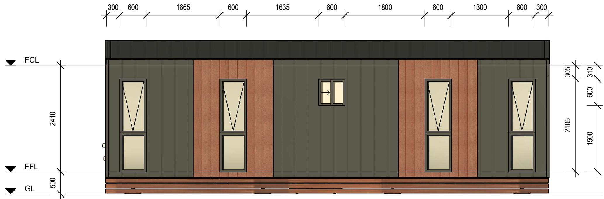
REAR ELEVATION (2)
