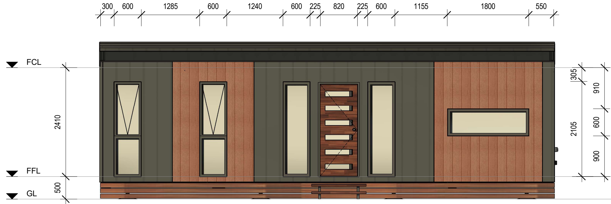
FRONT ELEVATION (1)
