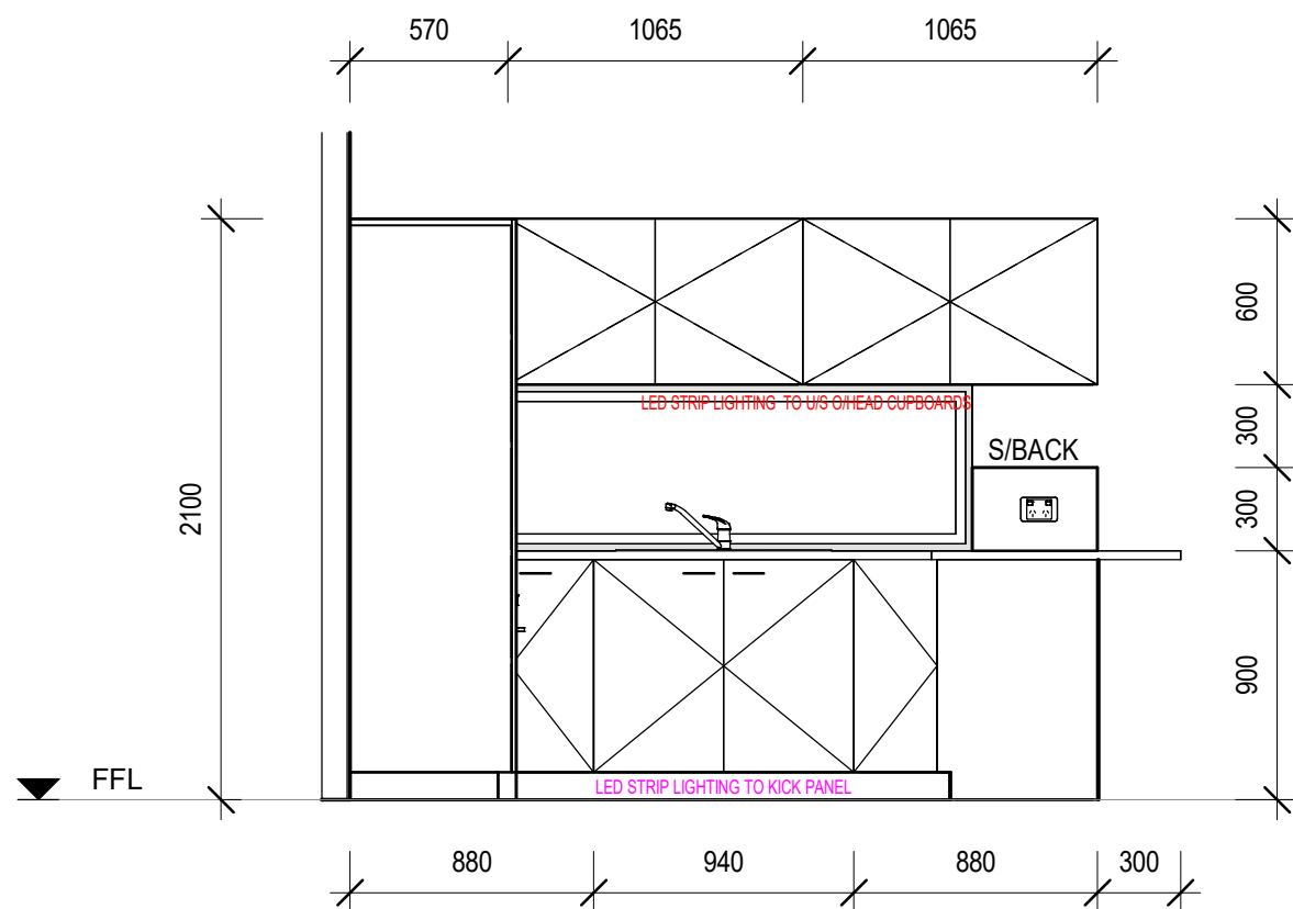
KITCHEN JOINERY - ELEVATION 1 (KE1)
