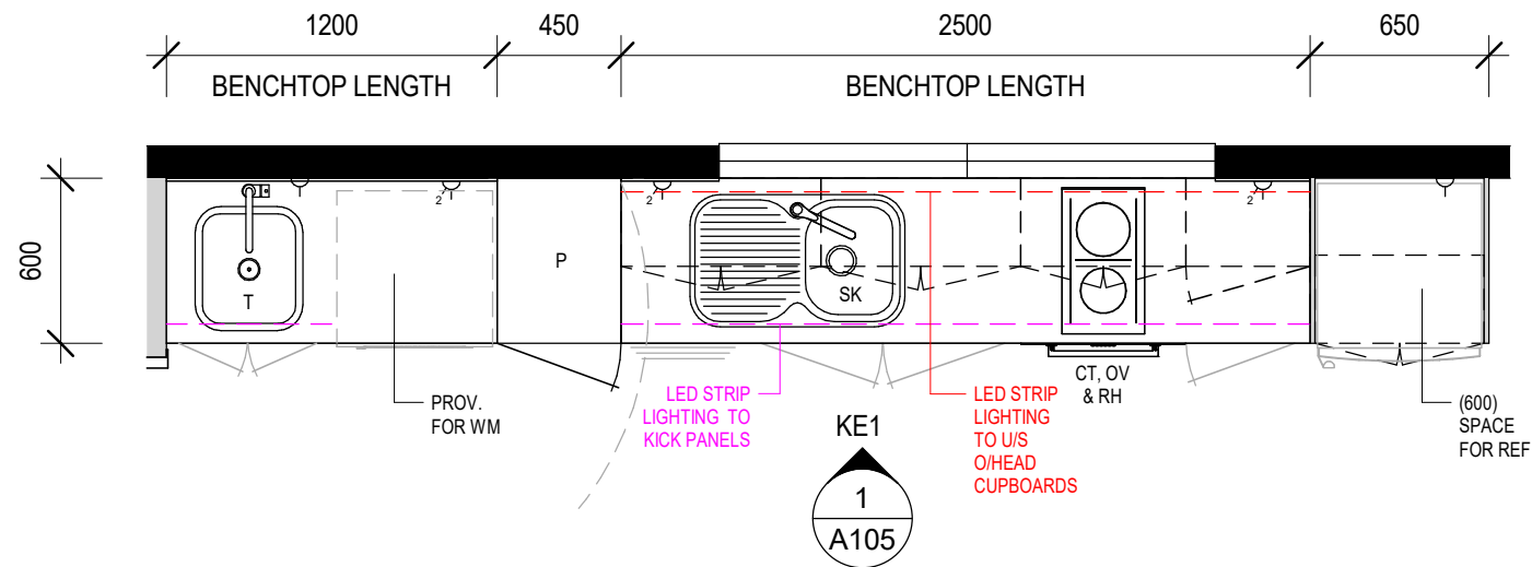
KITCHEN & LAUNDRY JOINERY - PLAN VIEW
