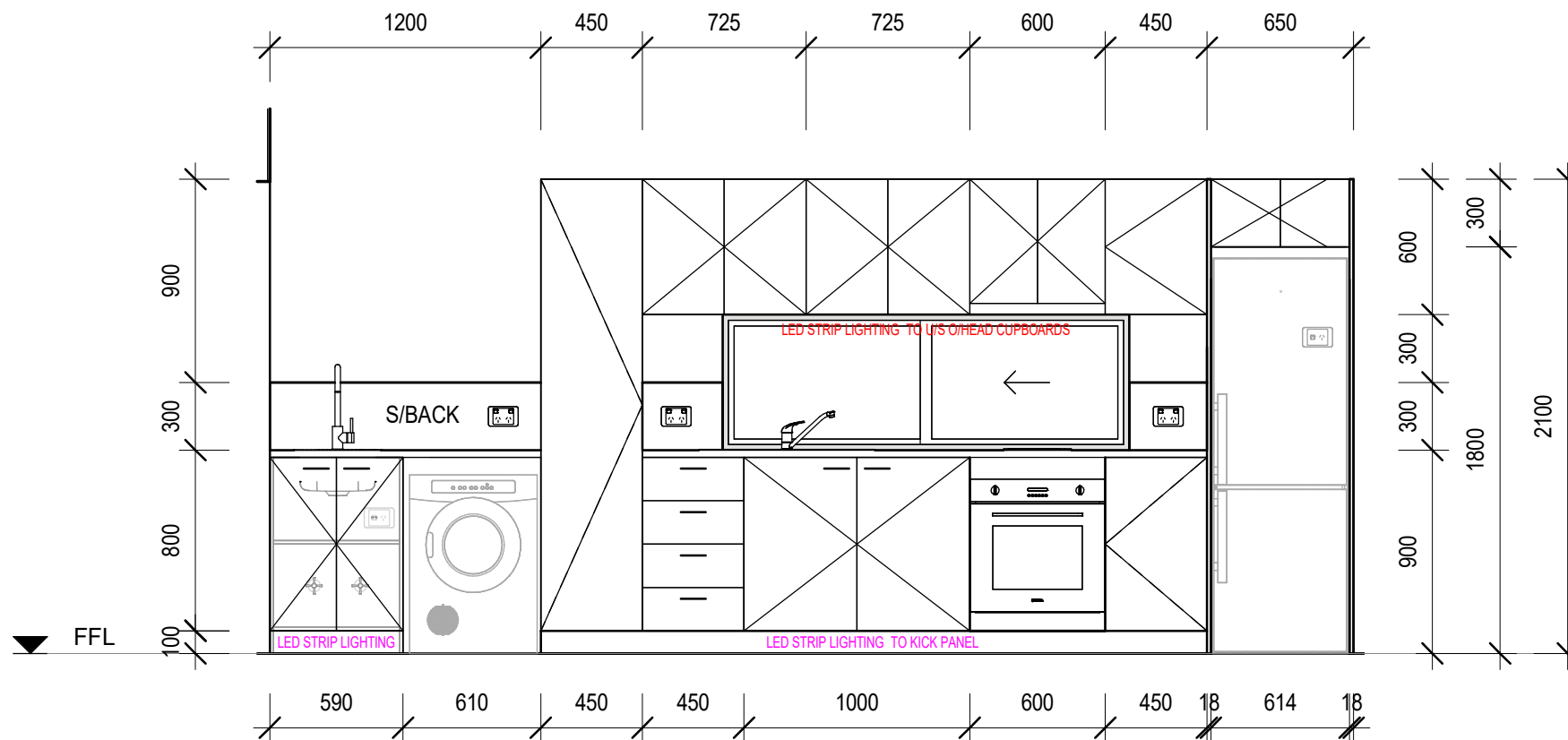
KITCHEN & LAUNDRY ELEVATION 1 (KE1)
