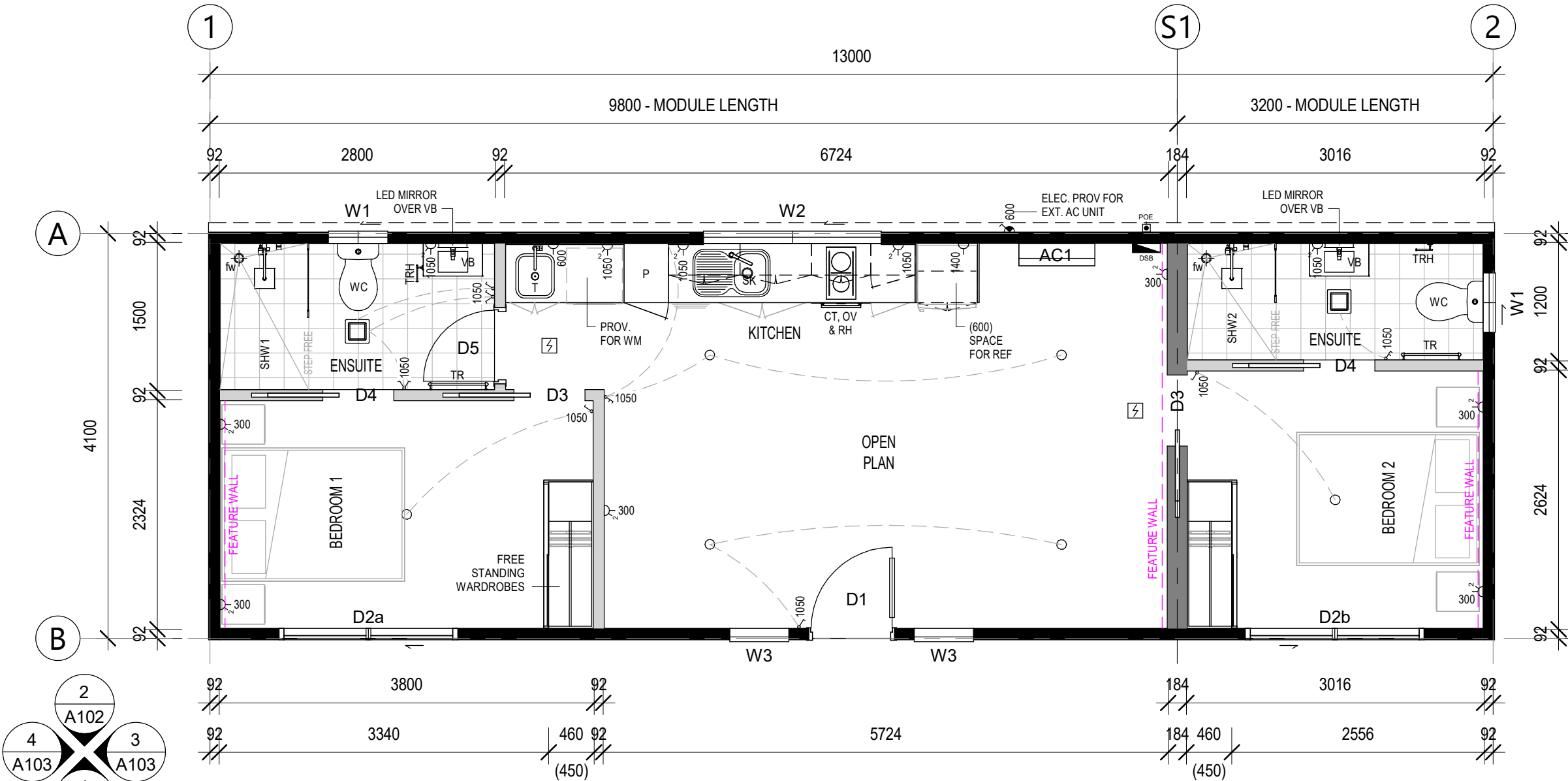
FLOOR PLAN
