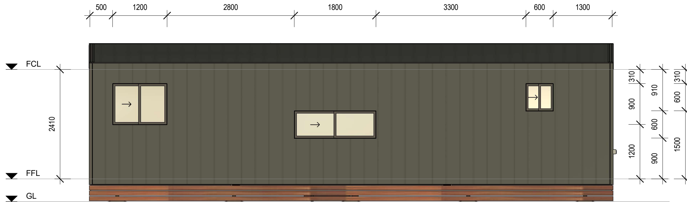
REAR ELEVATION (2)
