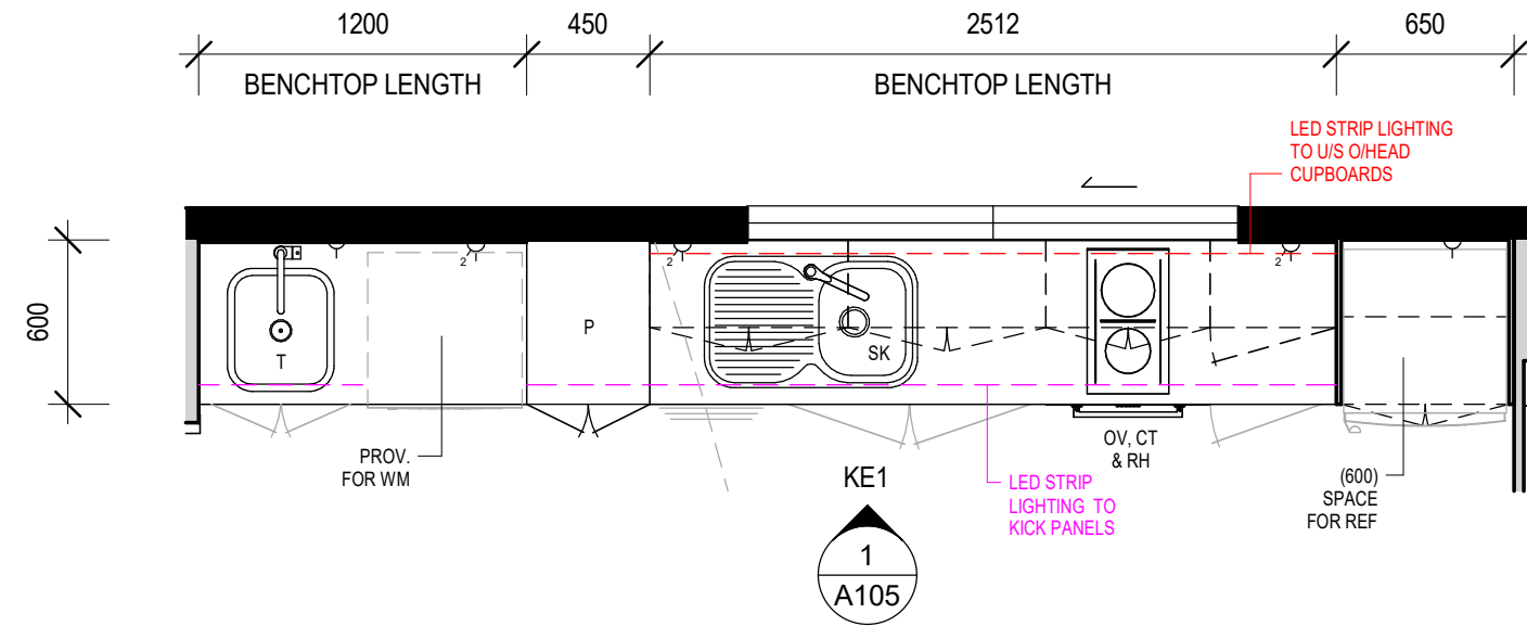
KITCHEN/LAUNDRY JOINERY - PLAN VIEW
