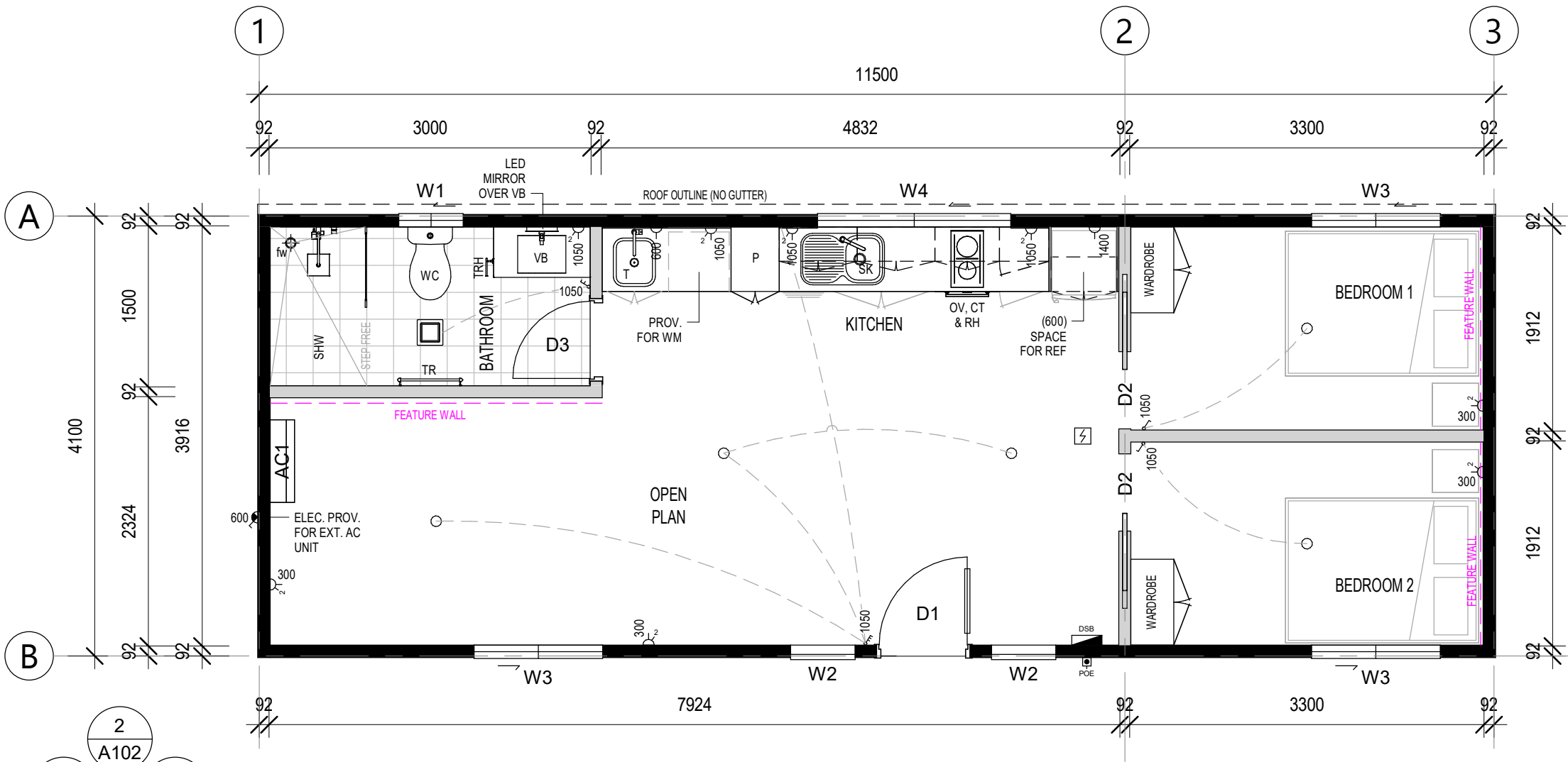
FLOOR PLAN
