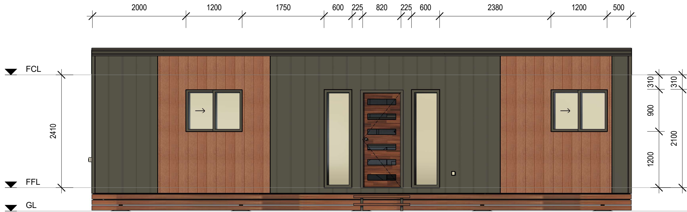
FRONT ELEVATION (1)
