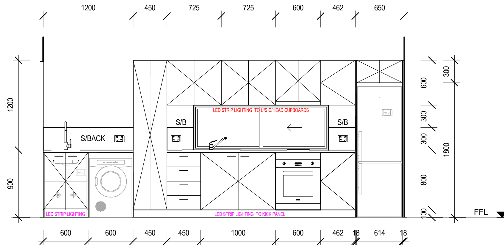
KITCHEN/LAUNDRY JOINERY ELEVATION 1 (KE1)
